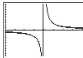
[0, \pi] by [-10, 10]
