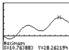
[0, 13] by [-20, 50]
