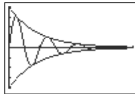
[0, 2\pi] by [-1, 1]
