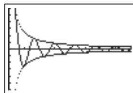
[0, 4\pi] by [-1.5, 1.5]
