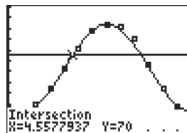
[0, 13] by [42, 88]
