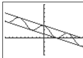
[-10, 10] by [-4, 8]
