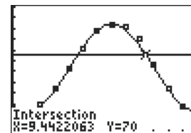
[0, 13] by [42, 88]
