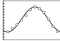
[0, 13] by [20, 90]
