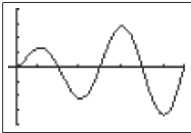
[-0.5, 4\pi] by [-4, 4]
