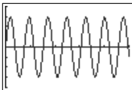
[0, 0.025] by [-2, 2]
