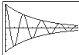
[0, 4\pi] by [-1, 1]
