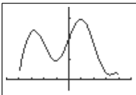
[-2.5, 2.5] by [-0.5, 3.5]
