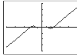
[-1, 1] by [-1, 1]
