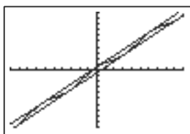
[-10, 10] by [-20, 20]
