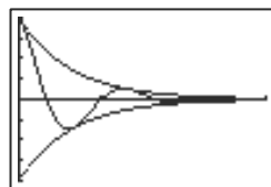
[0, 1.5\pi] by [-1, 1]
