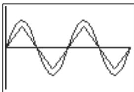
[0, 2\pi] by [-1.5, 1.5]
