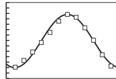
[0, 13] by [10, 80]
