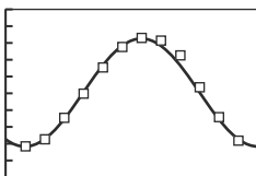
[0, 13] by [40, 90]
