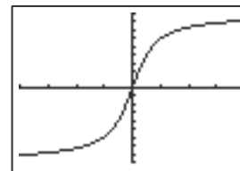
[-20, 20] [-90, 90]
