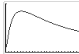
[0, 25] by [0, 55]
