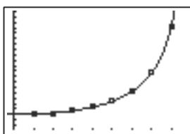
[-0.3, 8.7] by [2.32, 24]
